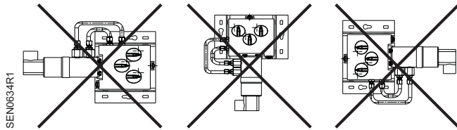
Figure 6. Unapproved Mounting Positions.
