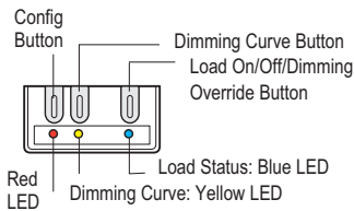
Button Selection Location and LEDs
