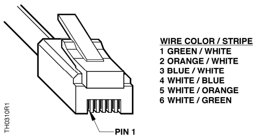
Figure 4. Terminating the RJ-11 Connector.
